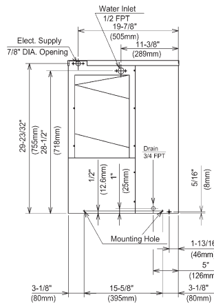
AIR-COOLED UNIT
