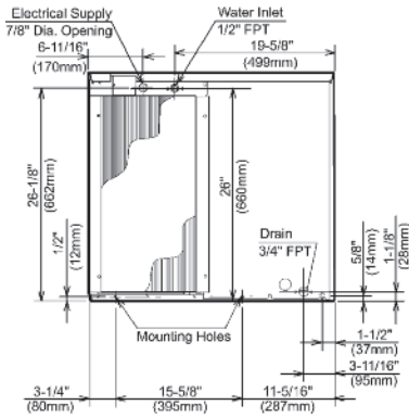
AIR-COOLED UNIT
