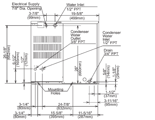
WATER-COOLED UNIT
