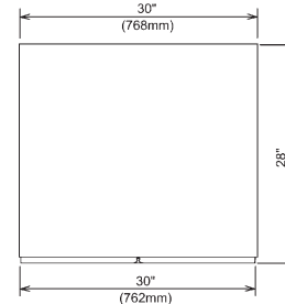
KMD-700MRH & MWH FRONT VIEW
