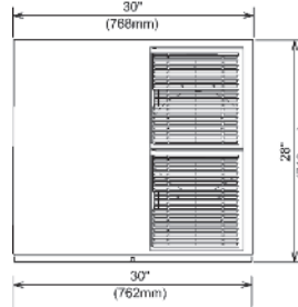
KMD-700MAH FRONT VIEW
